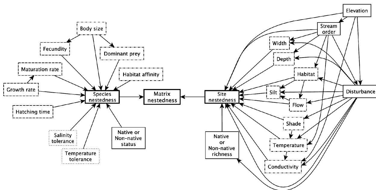
Fig. 1 The causal pathways, as specified using structural equations, by which species and site attributes were hypothesized to directly and indirectly affect the nested metacommunity structure of fishes in streams tributary to the San Francisco Bay.
