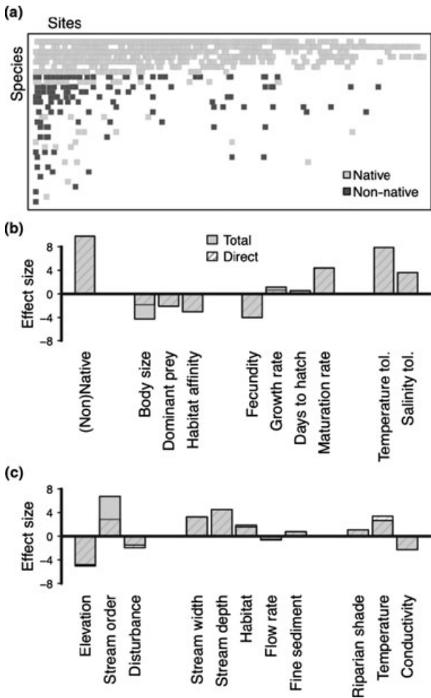
Fig. 2 (a) The incidence matrix of stream fish metacommunity, ordered by occupancy and richness, highlighting the importance of distinguishing between native and nonnative species. Below, total ( \beta_T ) and direct ( \beta_D ) effects of (b) species- and (c) site attributes on the species- and site nestedness of the metacommunity as revealed by the explicit consideration of their causal correlations using permutation-based gradient analysis. See Table 1 for variable explanations. Effect sizes indicate the change in nestedness expected when rows or columns are ordered by a focal variable in descending order, accounting for the ordering of secondary variables.
