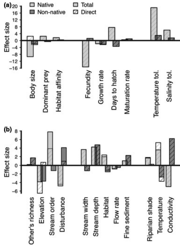
Fig. 3 The total and direct effects of (a) species- and (b) site attributes on the nested community structure of native and non-native fishes as revealed by the explicit consideration of their causal correlations using the permutation-based gradient analysis.
